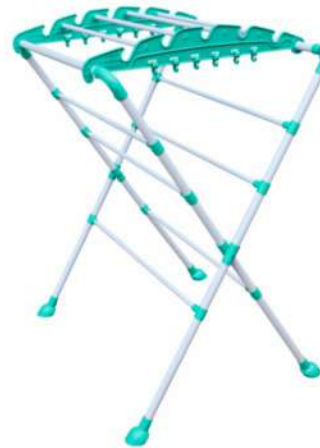
Mini Jumbo | Cat No. : CD-002 Opening Size : 957mm X 734mm X 1321mm Closing Size : 940mm X 1140mm X 180mm Master Box: 4 Pcs.
